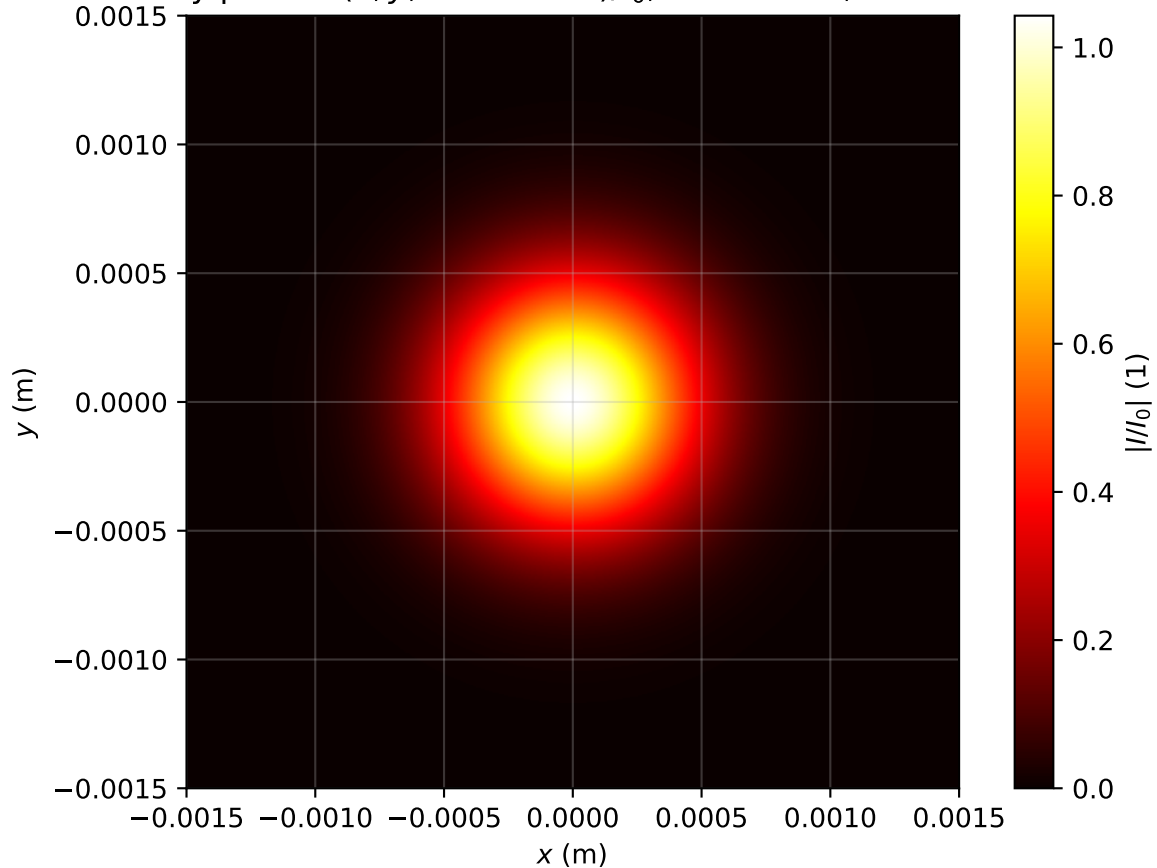
Intensity profile I(x, y, z = 0.239m)/I_0 , Pin=1.0Pcr, artificial time
